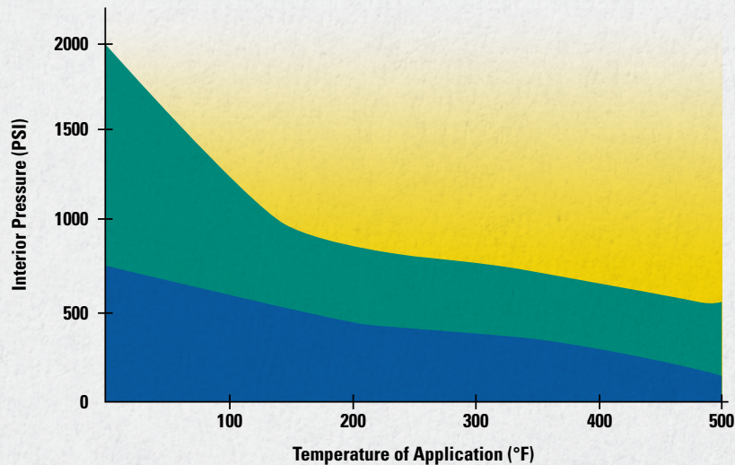
SEALEX® Pressure/Temperature Curves
